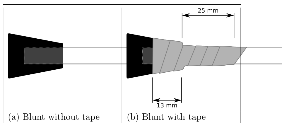
Figure 10. Blunt attachment
